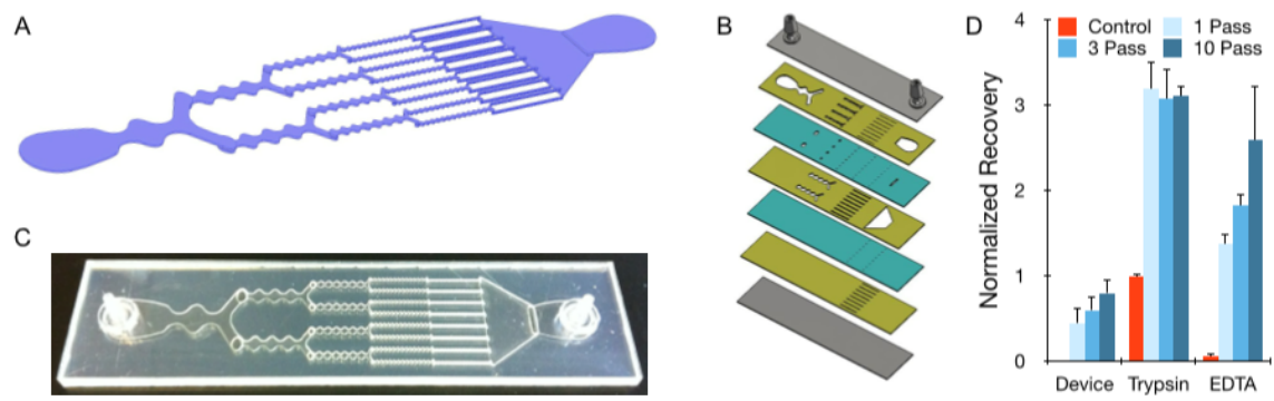
Figure: Microfluidic dissociation device. (A) Schematic of the branching channel design. (B) Side view showing the 7 layers (3 channel, 2 via, and 2 end caps). (C) Fabricated prototype. (D) Device results for HCT 116 spheroids when used alone or after brief (5 min) trypsin or EDTA treatments.
